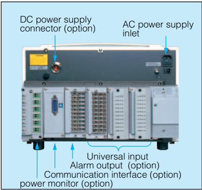
Rear panel of the stand-alone model
